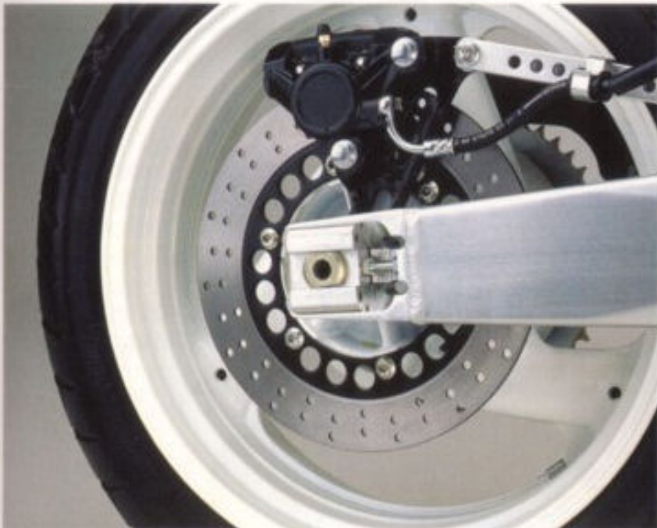
Rear brake/chain pullers A 267 mm drilled disc and a twin pot caliper at the rear provide added stopping power and solid 'feel'. The YZF-style drive chain pullers offer quick chain tensioning with accurate positioning of the rear axle.
