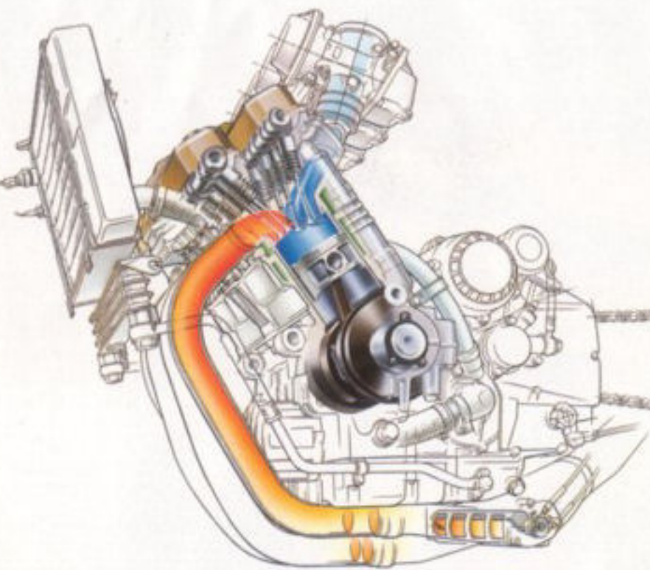
Five-valve heads Unique in the motorcycle world, the FZR's three inlet and two exhaust valves per cylinder improve gas flow into and out of the combustion chambers to give better all-round performance. The result is a free revving yet torquy motor with unsurpassed top end.
