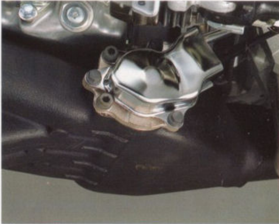
EXUP Driven by a microprocessor-controlled servo-motor, Yamaha's revolutionary EXUP (Exhaust Ultimate Power Valve) system controls gas pressure waves in the exhaust system, significantly boosting low- to mid-range torque.
