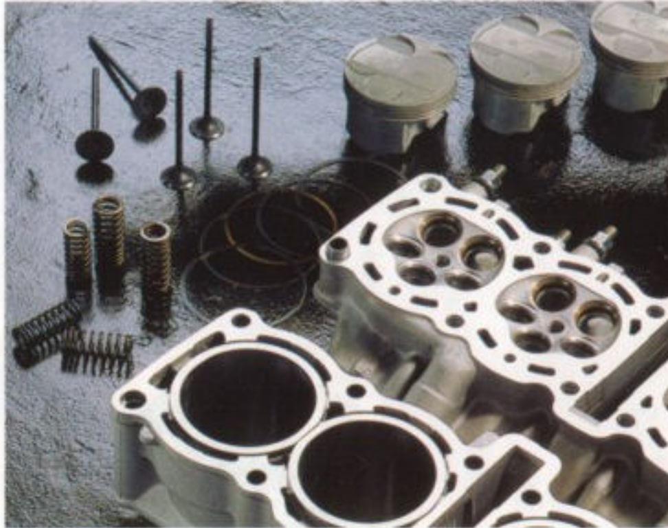
Five-valve heads Unique in the motorcycle world, the FZR's three inlet and two exhaust valves per cylinder improve gas flow into and out of the combustion chambers to give better all-round performance. The result is a free revving yet torquy motor with unsurpassed top end.
