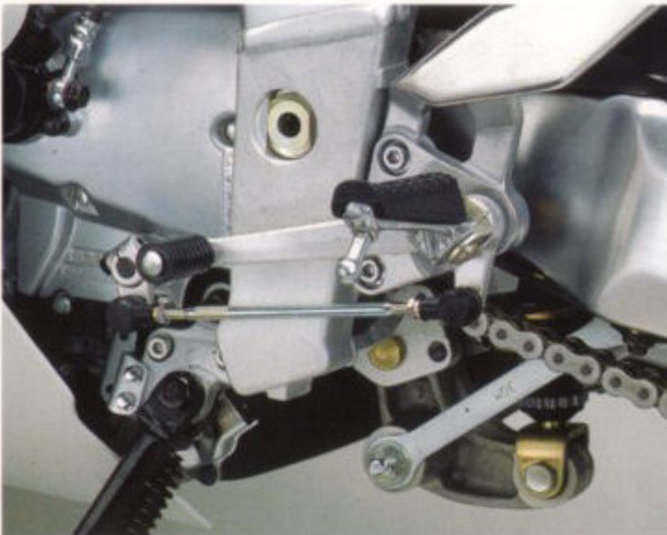
Gearbox Counter-tapered engagement dogs give the FZR one of the smoothest shifting gearboxes in its class. Five carefully chosen ratios from 2.571 up to 1.037 enable the rider to make the most of the potent 1003 cc motor.
