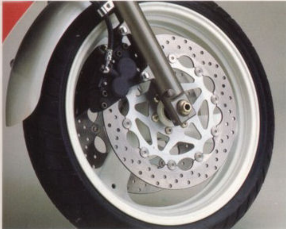
Front brake Braking power up front is supplied by opposed, different sized four-piston calipers working on twin 320 mm floating discs. Together with another disc at the rear, this is one of the most powerful set-ups available on two wheels.
