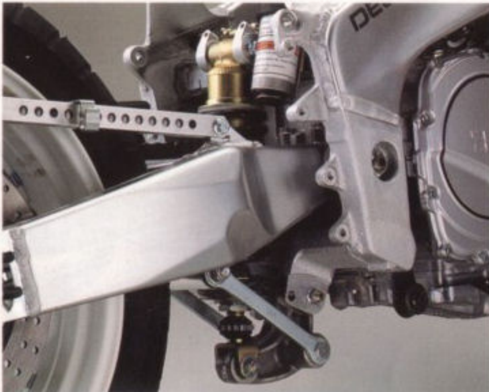
Rear suspension Adjustable for spring pre-load and compression damping, the Monocross gas/oil rear shock gives a full 130 mm of rear wheel travel. Light alloy Deltabox swinging arm features triangulated design for superior rigidity.
