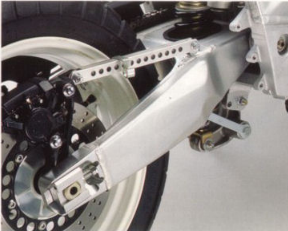
Deltabox swinging arm Constructed in aluminium, the Deltabox swinging arm is triangulated for maximum rigidity and light weight. It reduces the machine's unsprung weight and improves rear-wheel roadholding.
